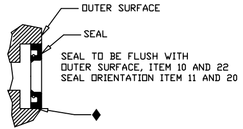
PARTIAL SECTION VIEW A
